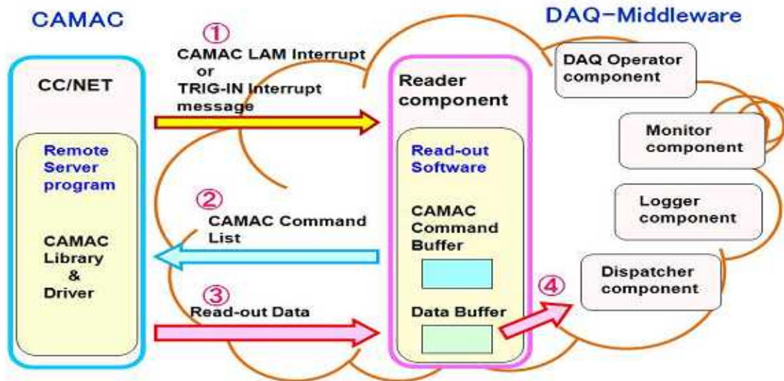
Figure 7. Data passing between CAMAC and the DAQ-Middleware.
