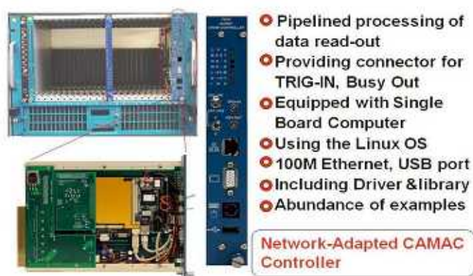
Figure3. Brief overview of the CC/NET.
